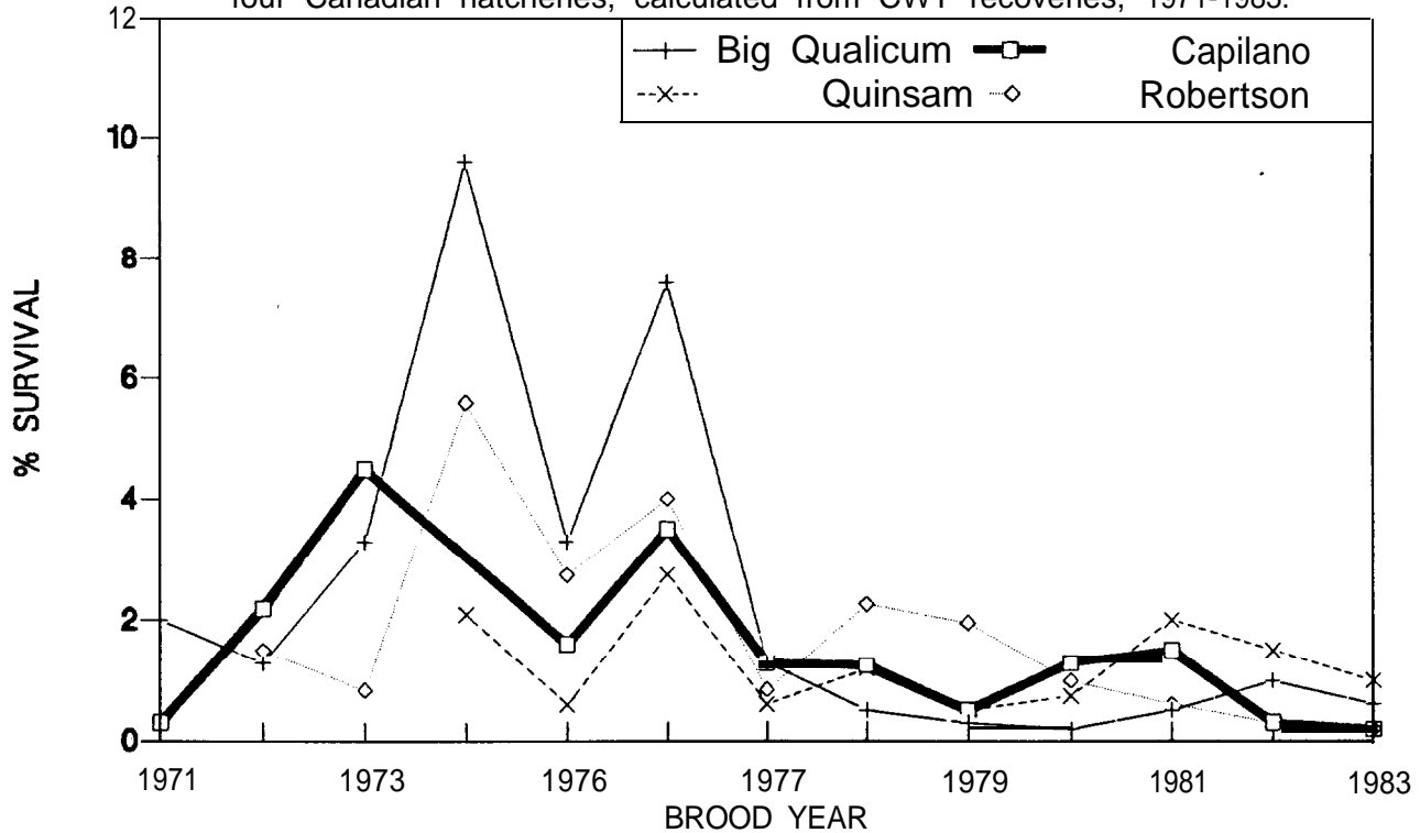
Figure 5-5 Trends of total survivals of hatchery chinook salmon for four Canadian hatcheries, calculated from CWT recoveries, 1971-1983.*
